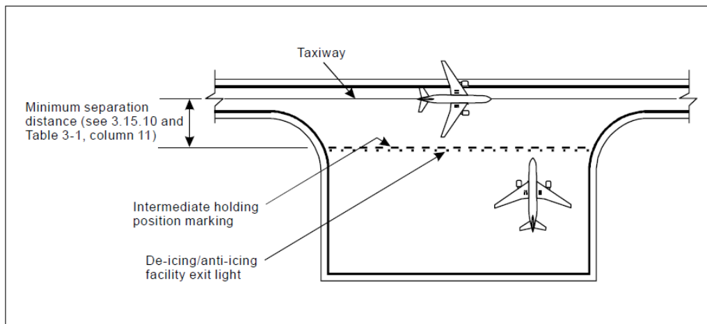
Figure 5-24. Typical remote de-icing/anti-icing facility
