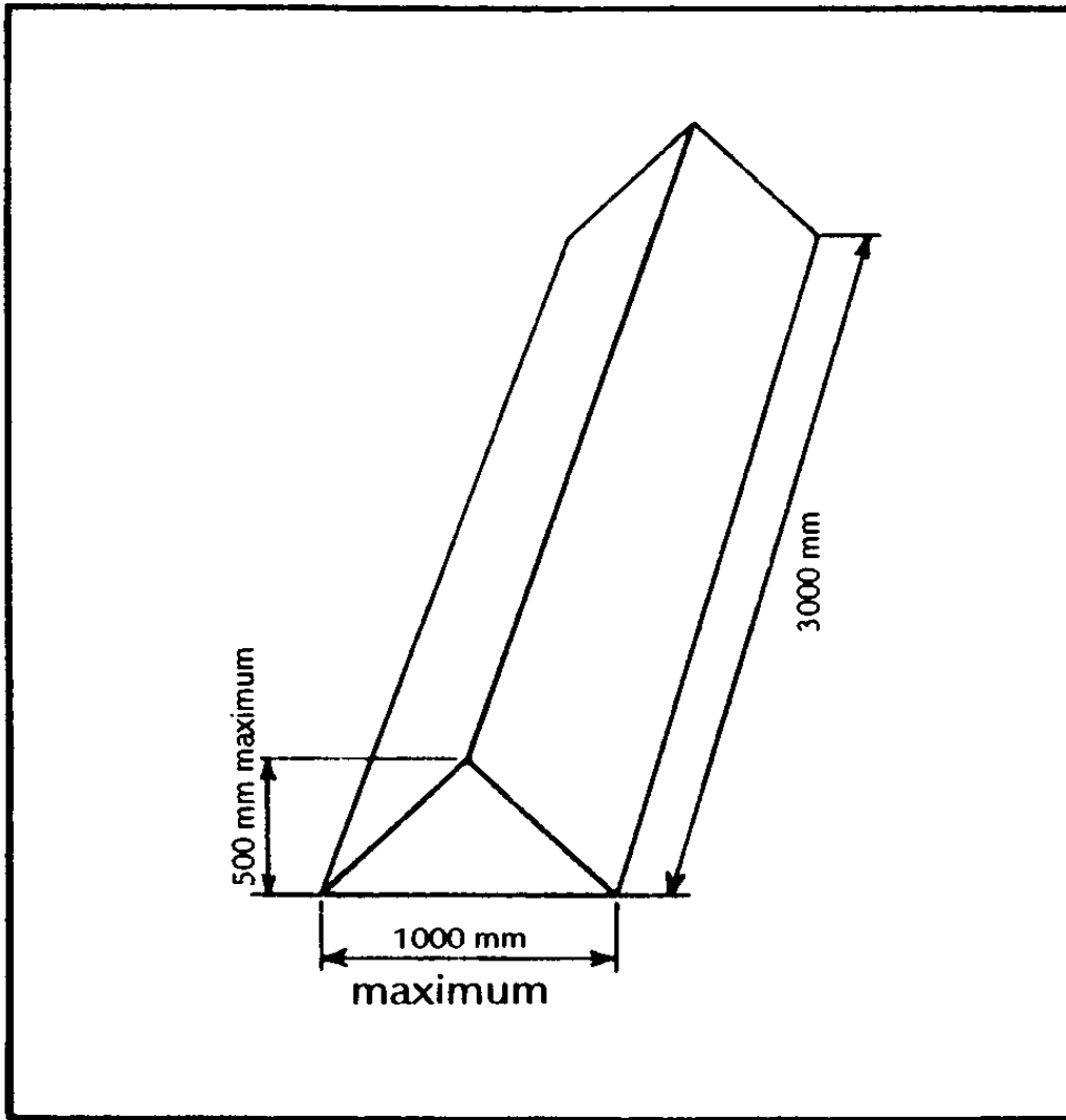
Figure 5-32 Marker Board
