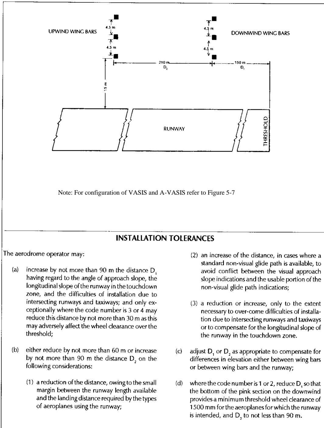
Figure 5-18. Installation of wing bars for VASIS and AVASIS
